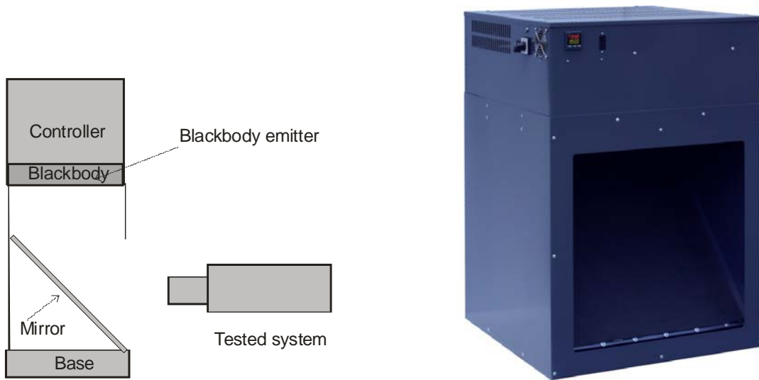
Fig.1. Block diagram and photo of the ULAB blackbody
