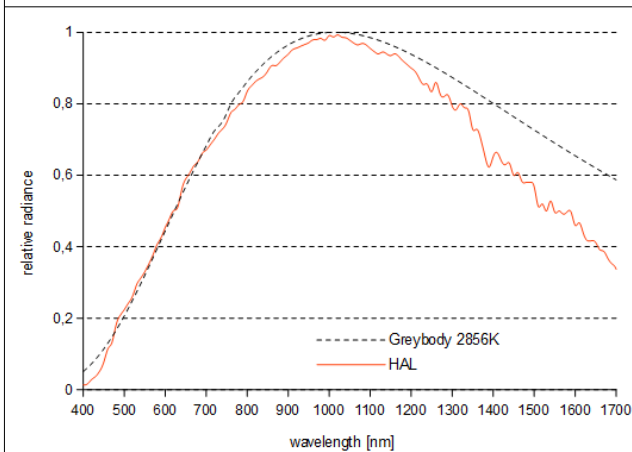
Fig.2. Relative spectrum of SEM1 light source
