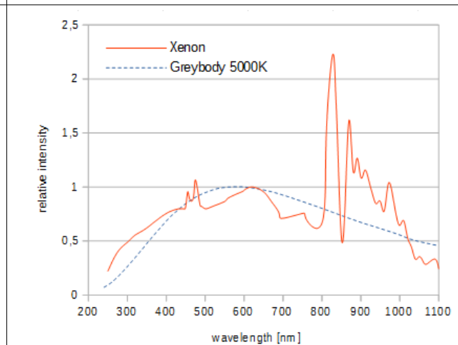
Fig.4. Relative spectrum of SEM2 light source
