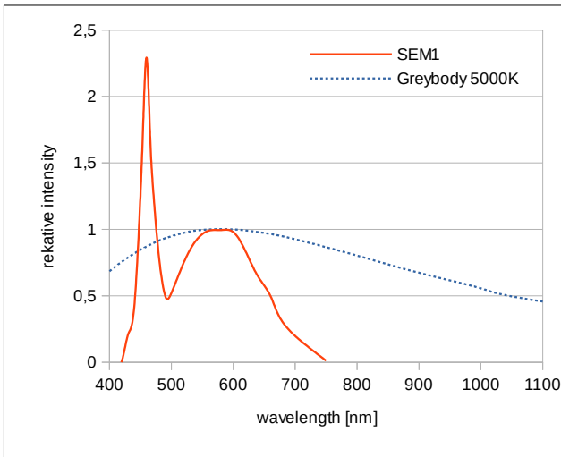
Fig.2. Relative spectrum of SEM1 light source
