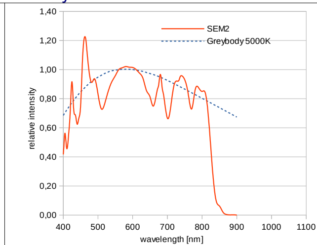
Fig.4. Relative spectrum of SEM2 light source
