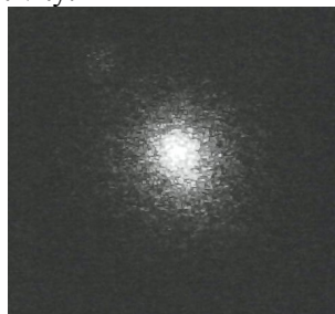
Fig.2. Image of illuminated field by laser illuminator of poor illumination uniformity
