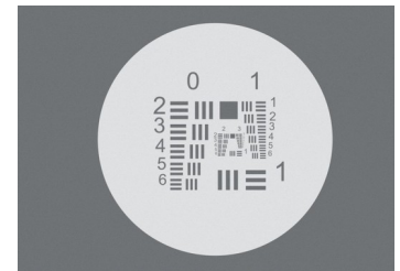
Fig.2. Image of USAF 1951 target generated by tested TV camera during MRC measurements
