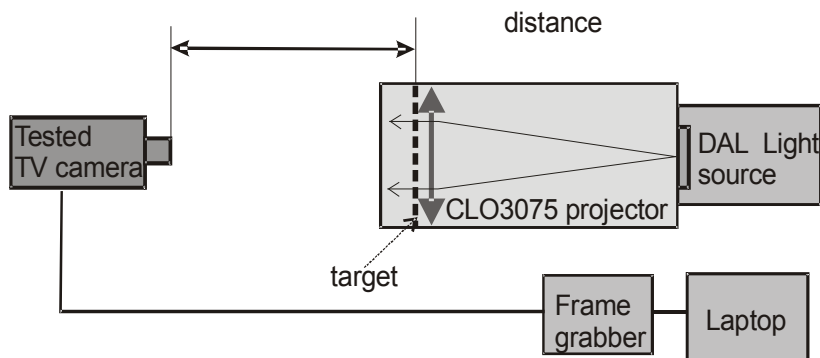
Fig.2. Block diagram of the LOF measuring set
