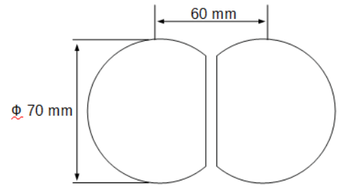
Fig. 2. Optical aperture of LTE station
