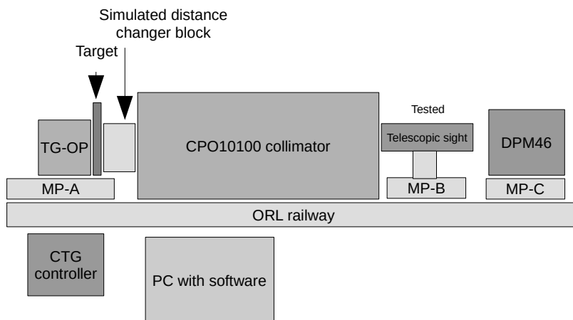
Fig. 3. Simplified block diagram of OPO test station
